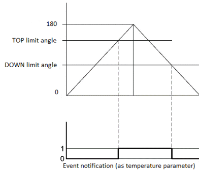
Fig. 3 The angle control mode demonstration.
