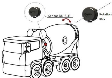
Fig. 2 Installation of the DU-BLE on the cement-mixer in vertical rotation control mode.
