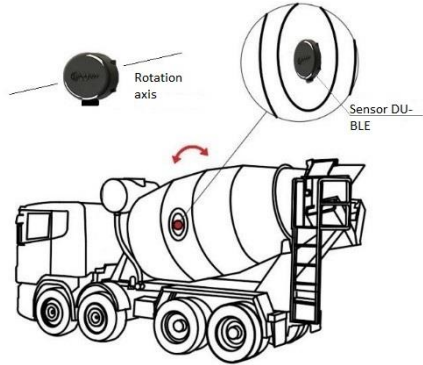
Fig. 1 Installation of the DU-BLE on the cement-mixer in vertical rotation control mode.
