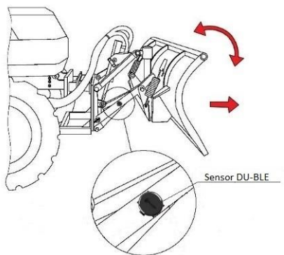
Fig.6. Installation of the DU-BLE on plow-type devices
